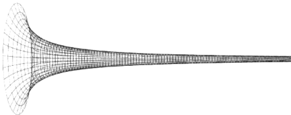
Figure 1. Gabriel's Horn.
